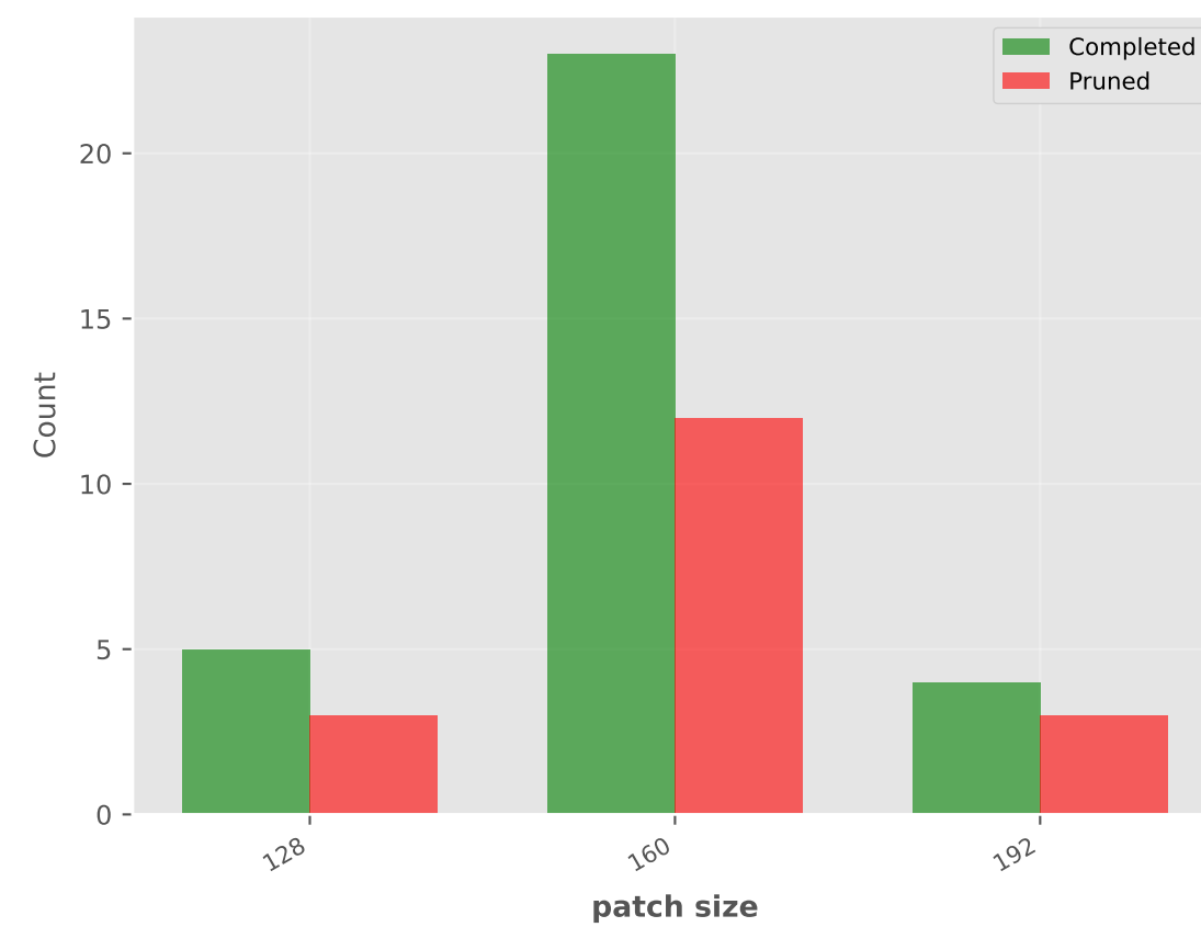
patch size: Completed vs Pruned
