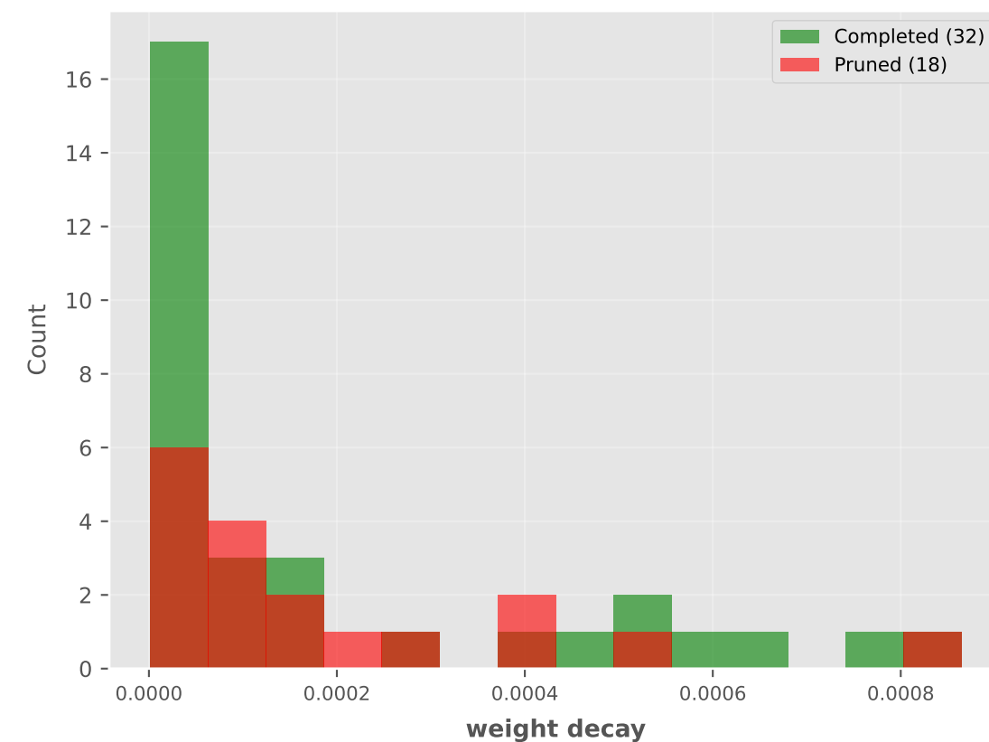
weight decay: Completed vs Pruned
