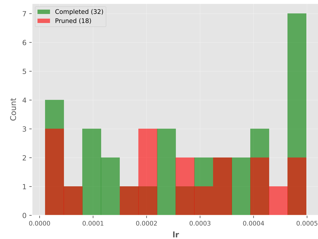
lr: Completed vs Pruned
